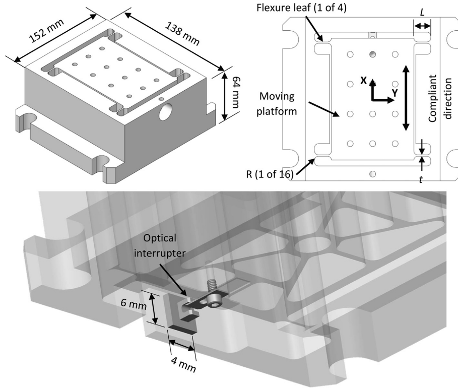
Fig. 1. CMD design and optical interrupter placement.
