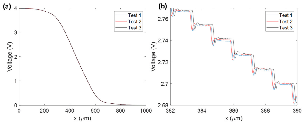
Fig. 2. Optical knife edge sensor calibration. The displacement sensitivity was determined to be 80 \mu\text{m}/\text{V} within the linear range of operation.
