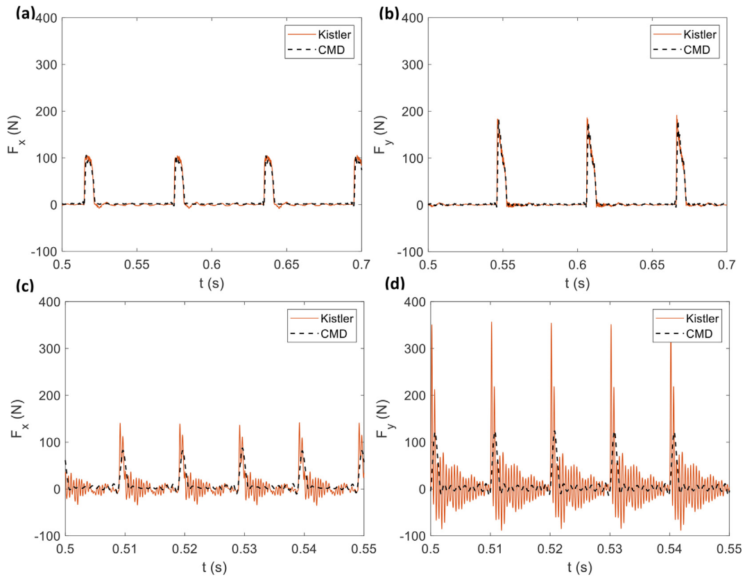
Fig. 6. Comparison of x and y direction cutting force signals for CMD (black dashed line) and Kistler 9257B (red solid line) for a spindle speed of 1000 rpm (a-b) and 6000 rpm (c-d), respectively. The distortion of the measured force signal by the Kistler 9257B dynamics is described using the measured force-to-force transmissibility FRFs for the dynamometer's x ( H_{xx} ) and y ( H_{yy} ) directions; see Fig. 7(a and b). Multiple modes are observed starting at approximately 700 Hz. The frequency content of the measured force has the expected peaks at the tooth passing frequency (100 Hz) and its harmonics. However, harmonics between 1000 Hz and 3000 Hz are artificially amplified by the dynamometer's vibration modes. To compensate for this amplification, the filtering technique described by Korkmaz et al. [12] was applied. The cutoff frequency, 1500 Hz, of the lowpass filter was selected such that the magnitude response of the final, inverse FRF filter is near unity at the limit of the dynamometer bandwidth, 5000 Hz. The filtered frequency content is displayed in Fig. 7(c-d), where the amplification has been effectively removed. Fig. 8 demonstrates good agreement between the compensated Kistler 9257B and CMD time domain cutting force results. (For interpretation of the references to colour in this figure legend, the reader is referred to the web version of this article.)
