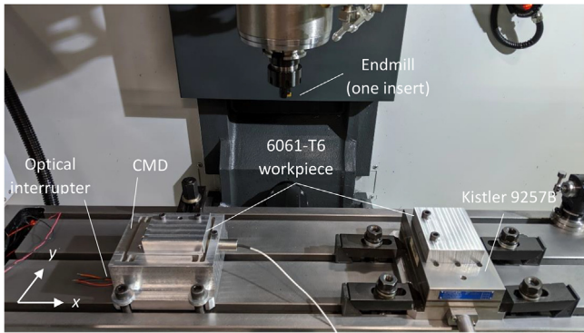
Fig. 3. Experimental setup showing the CMD, commercial dynamometer (Kistler 9257B), endmill, and workpieces.
