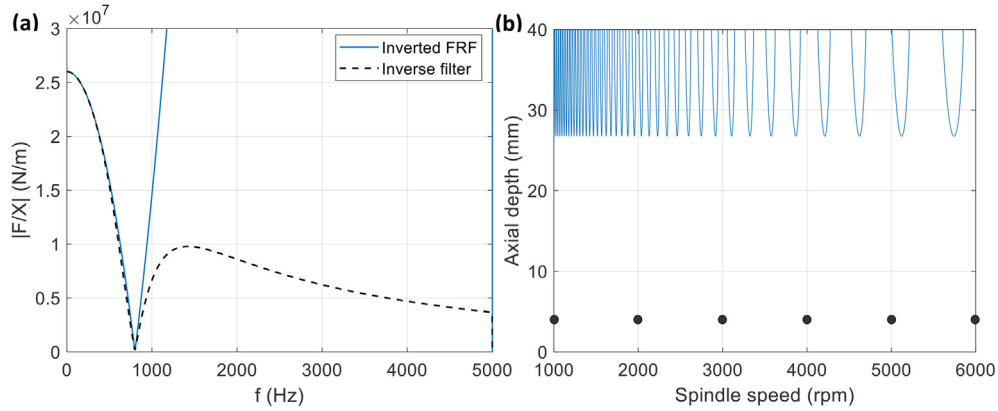
Fig. 5. Inverted FRF and inverse filter used to determine force from measured displacement (a). Stability map for CMD using a 6061-T6 aluminum workpiece, one insert endmill, and 10% radial immersion down milling. The test points are identified by solid circles.
