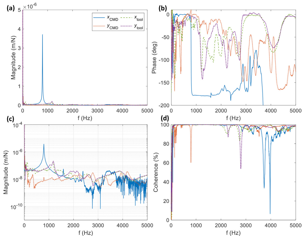
Fig. 4. Linear magnitude (a), phase (b), semi-logarithmic magnitude (c), and coherence (d) components of the CMD and tool FRFs.
