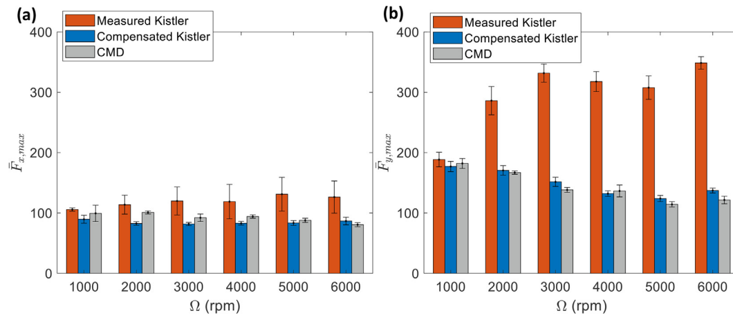
Fig. 8. Mean peak x force (a) and y force (b) values for the CMD (gray), Kistler 9257B (red), and compensated Kistler 9257B (blue). Error bars indicate 95% confidence intervals. (For interpretation of the references to colour in this figure legend, the reader is referred to the web version of this article.)
