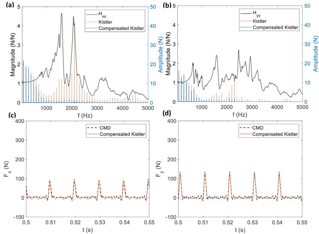
Fig. 7. Kistler 9257B force-to-force transmissibility FRF magnitudes for the x (a) and y (b) directions (black solid line) and force frequency content: measured (red solid) and compensated (blue dashed). Cutting force for compensated Kistler 9257B (red solid line) and CMD (black dashed) at a spindle speed of 6000 rpm for the x (c) and y (d) direction forces. Note that the scale matches Fig. 6. (For interpretation of the references to colour in this figure legend, the reader is referred to the web version of this article.)
