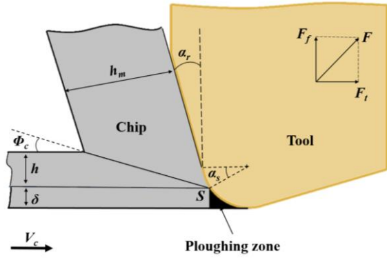
Figure 3. Schematic representation of ploughing
