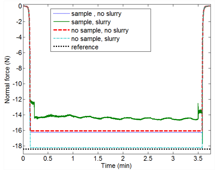
FIGURE 6 – NORMAL FORCE MEASUREMENT (PC1)
