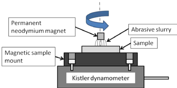
FIGURE 2 – SCHEMATIC OF EXPERIMENTAL SETUP
