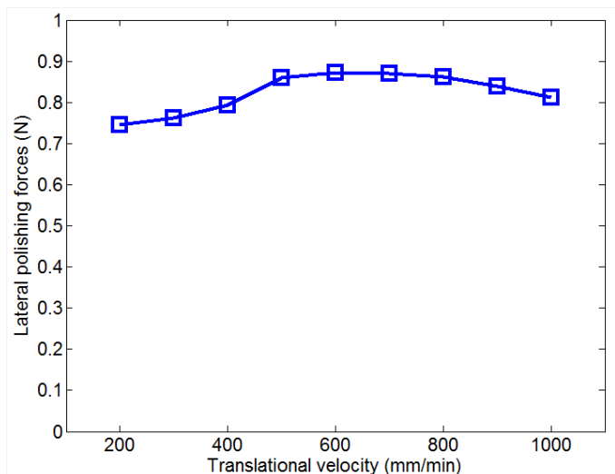
FIGURE 13 – EFFECT OF VELOCITY ON LATERAL FORCE
