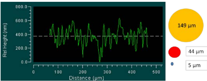
FIGURE 18 – SURFACE PROFILE SECTION WITH SCALED IRON PARTICLES (ACCORDING TO HORIZONTAL AXIS)
