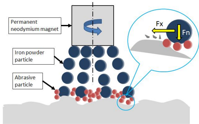
FIGURE 1 - MAF PROCESS (THE NORMAL, F_n , AND LATERAL, F_x , FORCE COMPONENTS ARE IDENTIFIED)
