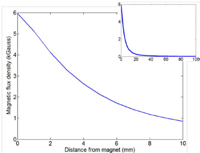
FIGURE 4 – MAGNETIC FLUX DENSITY FOR MAGNET ONLY
