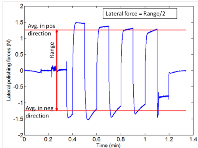
FIGURE 12 – LATERAL FORCE MEASUREMENT (PC1)
