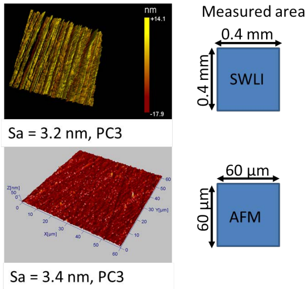
FIGURE 25 – COMPARISON OF SWLI (TOP) AND AFM (BOTTOM) MEASUREMENTS
