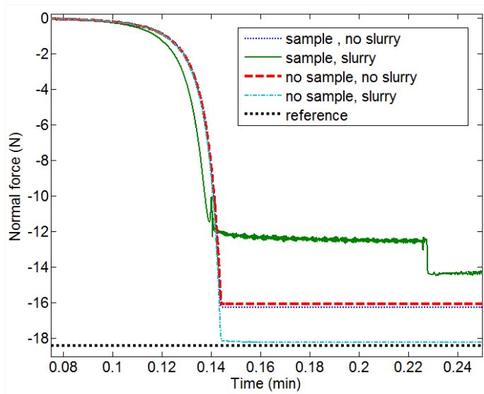
FIGURE 8 – NORMAL FORCE (APPROACH)
