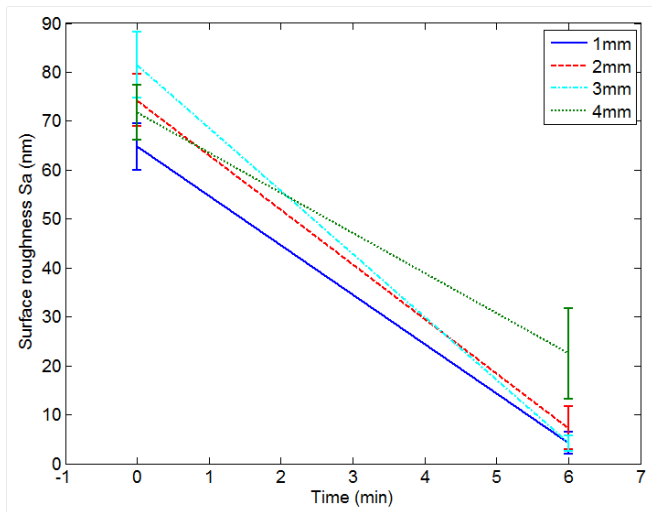
FIGURE 19 – SURFACE ROUGHNESS MEASUREMENTS FOR VARYING WORKING GAP SIZE
