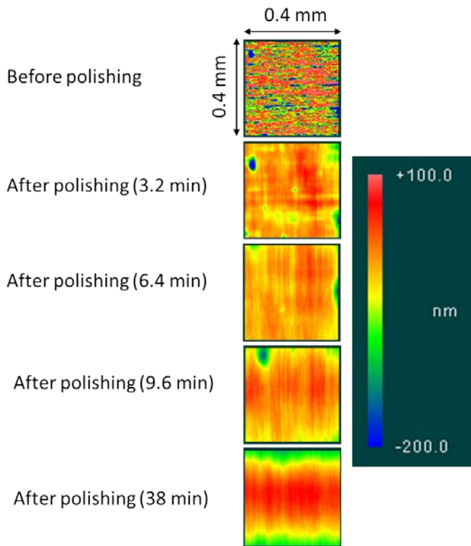
FIGURE 22 – VARIATION IN SURFACE TOPOGRAPHY AFTER POLISHING
