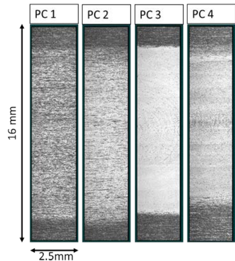
FIGURE 24 – LIGHT INTENSITY PLOT OF POLISHED AREA SECTIONS (DIFFERENT IRON PARTICLE SIZES)
