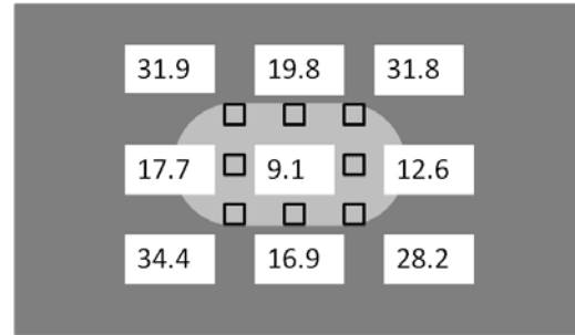
FIGURE 20 – SURFACE ROUGHNESS MEASUREMENTS FOR A WORKING GAP OF 4 MM (PC8).
