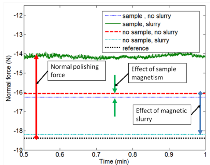
FIGURE 7 – NORMAL FORCE EFFECTS
