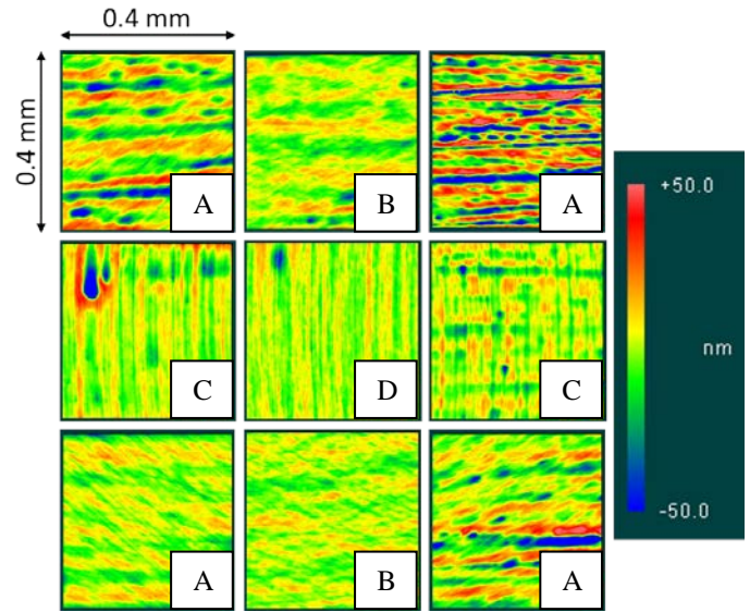
FIGURE 21 – DIRECTION OF LAY AFTER POLISHING
