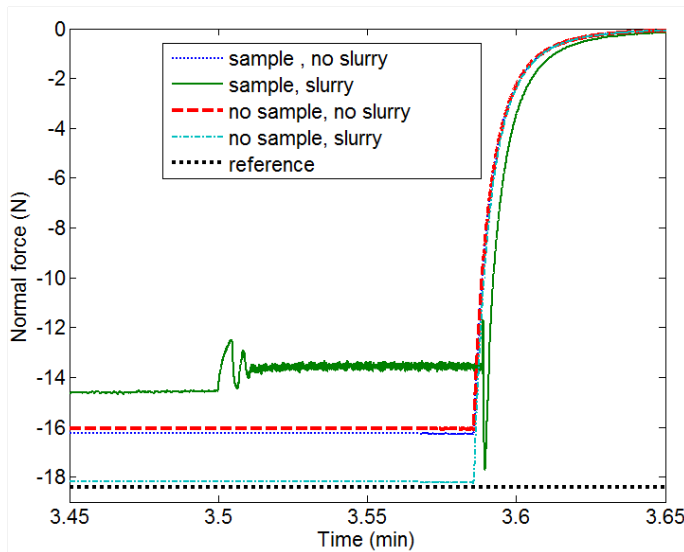
FIGURE 9 – NORMAL FORCE (RETRACT)
