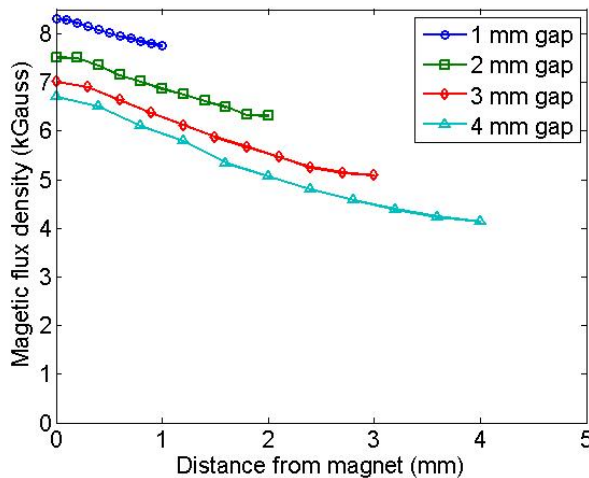
FIGURE 5 – MAGNETIC FLUX DENSITY WITH MOUNT
