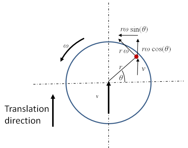
FIGURE 10 – VELOCITY COMPONENTS OF PARTICLE
