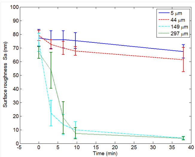
FIGURE 17 – SURFACE ROUGHNESS MEASUREMENT FOR VARYING IRON PARTICLE SIZE
