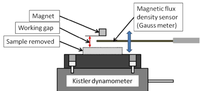
FIGURE 3 – SCHEMATIC OF EXPERIMENTAL SETUP FOR MEASURING MAGNETIC FLUX DENSITY
