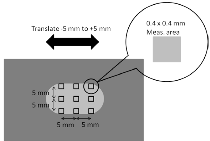
FIGURE 16 – SCHEMATIC OF SURFACE ROUGHNESS MEASUREMENTS
