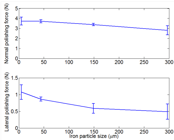
FIGURE 14 – POLISHING FORCE MEASUREMENTS FOR VARYING IRON PARTICLE SIZE
