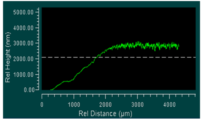
FIGURE 23 – CROSS-SECTIONAL VIEW OF POLISHED/UNPOLISHED INTERFACE
