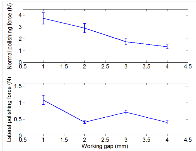
FIGURE 15 – POLISHING FORCE MEASUREMENTS FOR VARYING WORKING GAP SIZE
